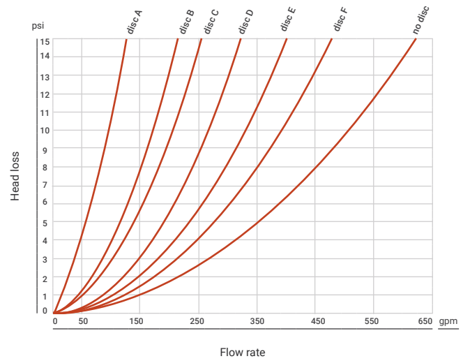
Circulating filter 4" (gpm)
