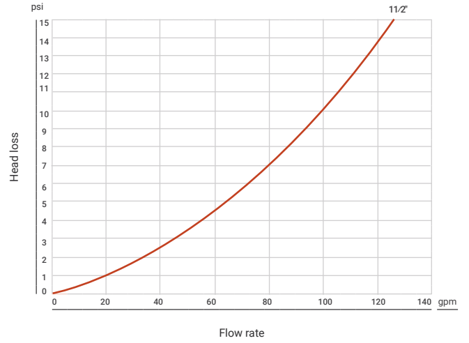
Circulating filter 1 1/2" (gpm)
