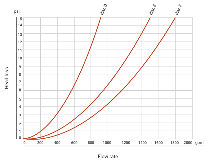
Circulating filter 8" (gpm)
