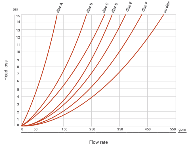
Circulating filter 3" (gpm)
