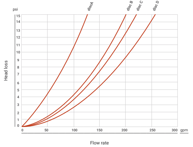
Circulating filter 2" (gpm)
