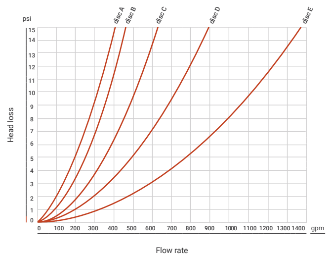
Circulating filter 6" (gpm)
